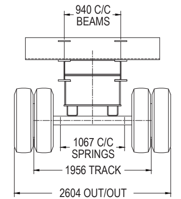
SECTION AT SUSPENSION MOUNT
